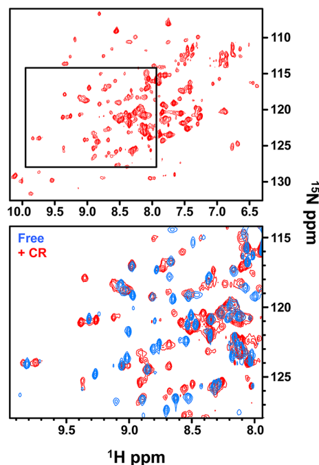
Figure 4. Comparison of CR-bound (red) and free (blue) Pot1pN ^1\text{H} – ^{15}\text{N} TROSY HSQC spectra obtained at 900 MHz. reveals differences upon CR binding, but no global changes or aggregation of Pot1pN. Boxed region of CR-bound spectrum in top panel is expanded below and superposed with free Pot1pN.
