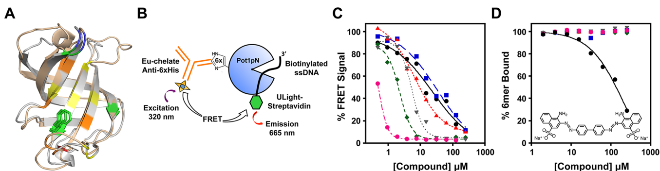
Figure 1. High-throughput screen and secondary validation of compounds identify a single inhibitor. (A) Pot1pN (wheat) superposed with OB1 of hPOT1 (white) shows structural similarity; the N- and C-terminal portions of each protein have been removed for clarity. Conserved residues on the ssDNA-binding surface are colored according to chemical character: aromatic (green), hydrophobic (yellow), polar (orange), acidic (red), and basic (blue). Pot1pN F88 (and corresponding hPOT1 F62) is shown as green sticks. Superposition was performed using LSQMAN 91 and the image was generated using MacPymol version 1.3. 92 (B) Schematic of the TR-FRET assay used to identify inhibitors of Pot1pN interaction with 6mer ssDNA. 6xHis-tagged Pot1pN is bound by the Eu-chelate anti-6xHis antibody (donor), which transfers energy to ULight-Streptavidin (acceptor) bound to biotinylated ssDNA. Excitation and FRET emission wavelengths are indicated. (C) Plot of the FRET-based dose-dependence of the activity of small molecules identified by the TR-FRET screen. Percent FRET signal is plotted as a function of compound concentration. (D) Plot of the dose-dependent inhibitory activity of the compounds from (C) by secondary filter-binding assay revealing only one compound (Congo red) that directly inhibits the Pot1pN/6mer interaction. Percent 6mer ssDNA bound is plotted as a function of compound concentration.
