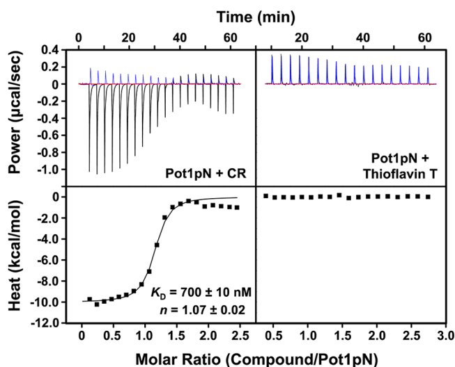
Figure 2. Pot1pN binds CR but not Thioflavin T. The left panels show baseline corrected raw ITC data (upper) for 1.2 mM CR titrated into buffer (blue) or 100 \mu M Pot1pN (black) and the reference-subtracted integrated heat of binding (lower). The right panels show baseline corrected raw ITC data (upper) for 2 mM Thioflavin T titrated into buffer (blue) or 100 \mu M Pot1pN (black) and the reference-subtracted integrated heat of binding (lower). K_D and n values for fitting triplicate Pot1pN/CR experiments to a one-site binding model are reported; errors are the standard error of the mean.
