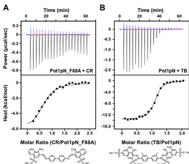
Figure 7. Mutation of Pot1pN and alteration of CR structure change the characteristics of binding. (A) Baseline corrected raw ITC data (upper) for 1.2 mM CR titrated into buffer (blue) or 100 \mu M Pot1pN_F88A and the reference-subtracted integrated heat of binding (lower). (B) Baseline corrected raw ITC data (upper) for 1 mM TB titrated into buffer (blue) or 103 \mu M Pot1pN and the reference-subtracted integrated heat of binding (lower). The structures of CR and TB are shown below for comparison. Titrations were performed at 20 °C with 21 injections. Integrated heat data were fit to a one-site binding model.
